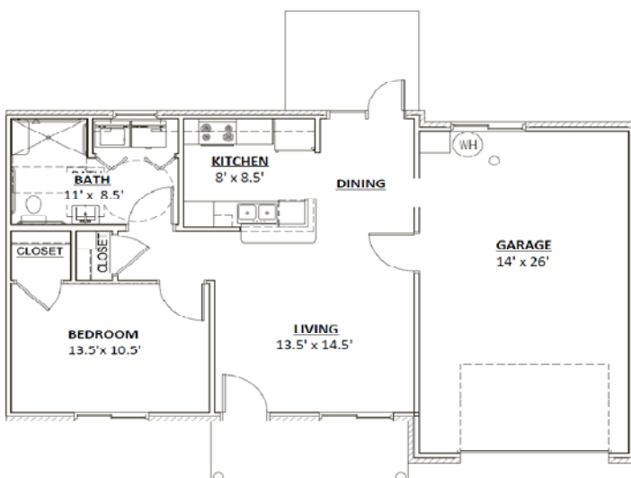
One Bedroom Villa (680 sq. ft.)
